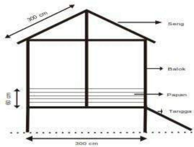
Tampak Samping
